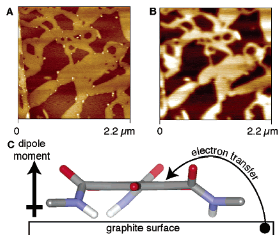
Figure 4. (A) 4.8 \mu\text{m}^2 AFM height image. (B) EFM 1\omega image of the same film. (C) Dipole and electron transfer in thin films of 1A .
